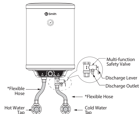
Figure 12 Installation Diagram
