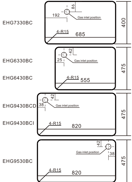
Bench cut-out size viewed from front of bench, i.e. control panel at front.
